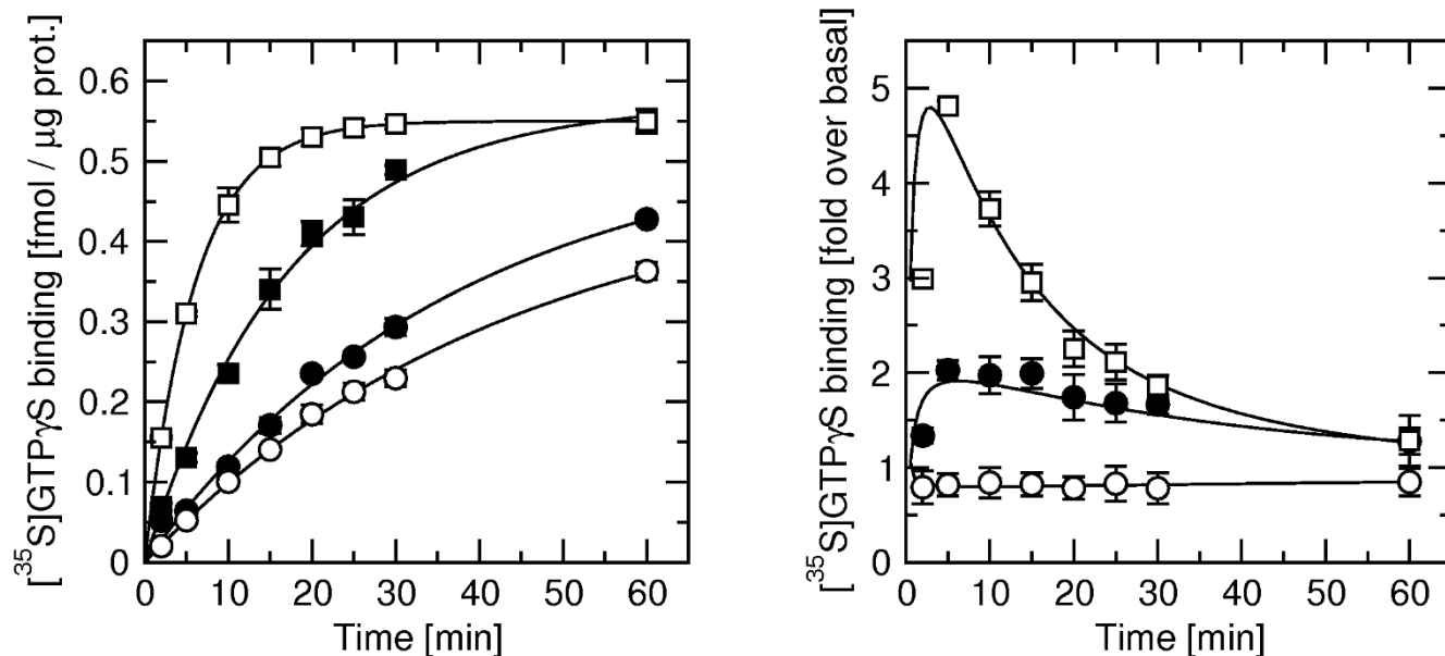
Figure 7 Effects of rapacuronium on kinetics of [ 35 S]GTPγS binding. Membranes were preincubated for 60 min in the presence (open symbols) or absence (closed symbols) of 1 μM rapacuronium. Then [ 35 S]GTPγS was added simultaneously with buffer (circles) or 10 μM ACh (squares). Incubations were terminated at the times indicated on the x-axis. The increase of specific [ 35 S]GTPγS binding is expressed as fmol per μg of protein (left) and as fold increase of specific binding under basal conditions (right). Data are means ± SE of values from 3 independent experiments performed in quadruplicates.
