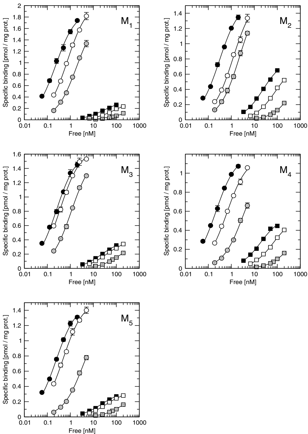
Figure 1 Saturation binding of [^3\text{H}]\text{NMS} and [^3\text{H}]\text{ACh} . Specific binding of [^3\text{H}]\text{NMS} (circles) and [^3\text{H}]\text{ACh} (squares) to membranes from CHO cells expressing individual subtypes of muscarinic receptors is plotted against the concentration of free radioligand. Binding of radioligand in the absence (closed symbols) and presence of 10 \mu\text{M} (open symbols) or 100 \mu\text{M} (hatched symbols) rapacuronium, respectively. Data are means \pm SE from 3 independent experiments performed in quadruplicates. Curves are fits of Eq. 1 to data. Binding parameters are summarized in Table 1.
