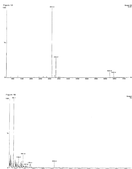
Figure 1 Determination of Domoic acid by electrospray mass spectrometry. (A) The electrospray mass spectrometry spectrum of 12.5 mM Domoic acid shows that the dominate ion in the spectrum is m/z 312.2, the pseudomolecular ion [M+H]^+ of Domoic acid, demonstrating that undegraded Domoic acid was present in the 12.5 mM stock solution; (B) The electrospray mass spectrometry spectrum of 0.0025 mM Domoic acid, the highest dilution used in the experiments, also shows the presence of undegraded Domoic acid.
